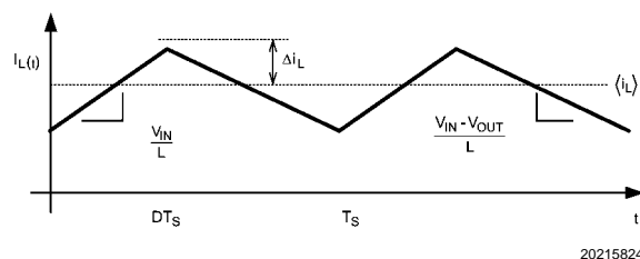
FIGURE 4. Inductor Current
