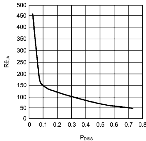
FIGURE 14. R θJA vs Internal Dissipation for the LLP-6 and eMSOP-8 Package
