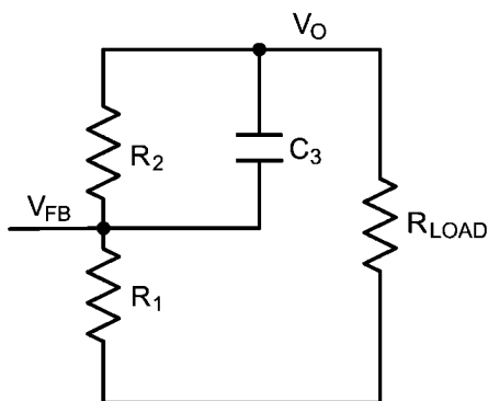
FIGURE 5. Setting Vout
