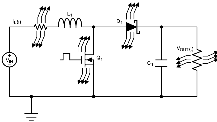
FIGURE 11. Thermal Schematic
