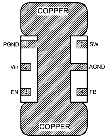
FIGURE 19. PCB Dog Bone Layout
