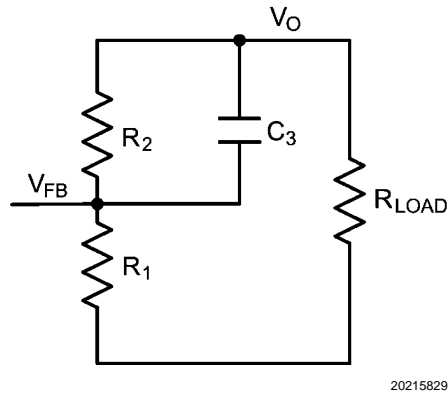
FIGURE 8. Setting External Pole-Zero
