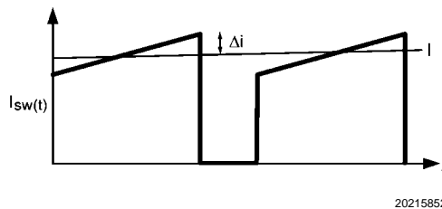
FIGURE 13. LM2735 Switch Current
