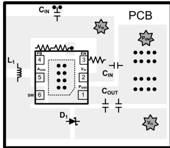
FIGURE 9. Boost PCB Layout Guidelines
